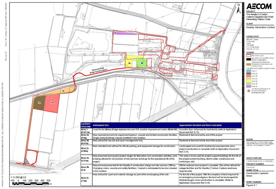
Figure 5.2: Selected Construction Laydown Areas
